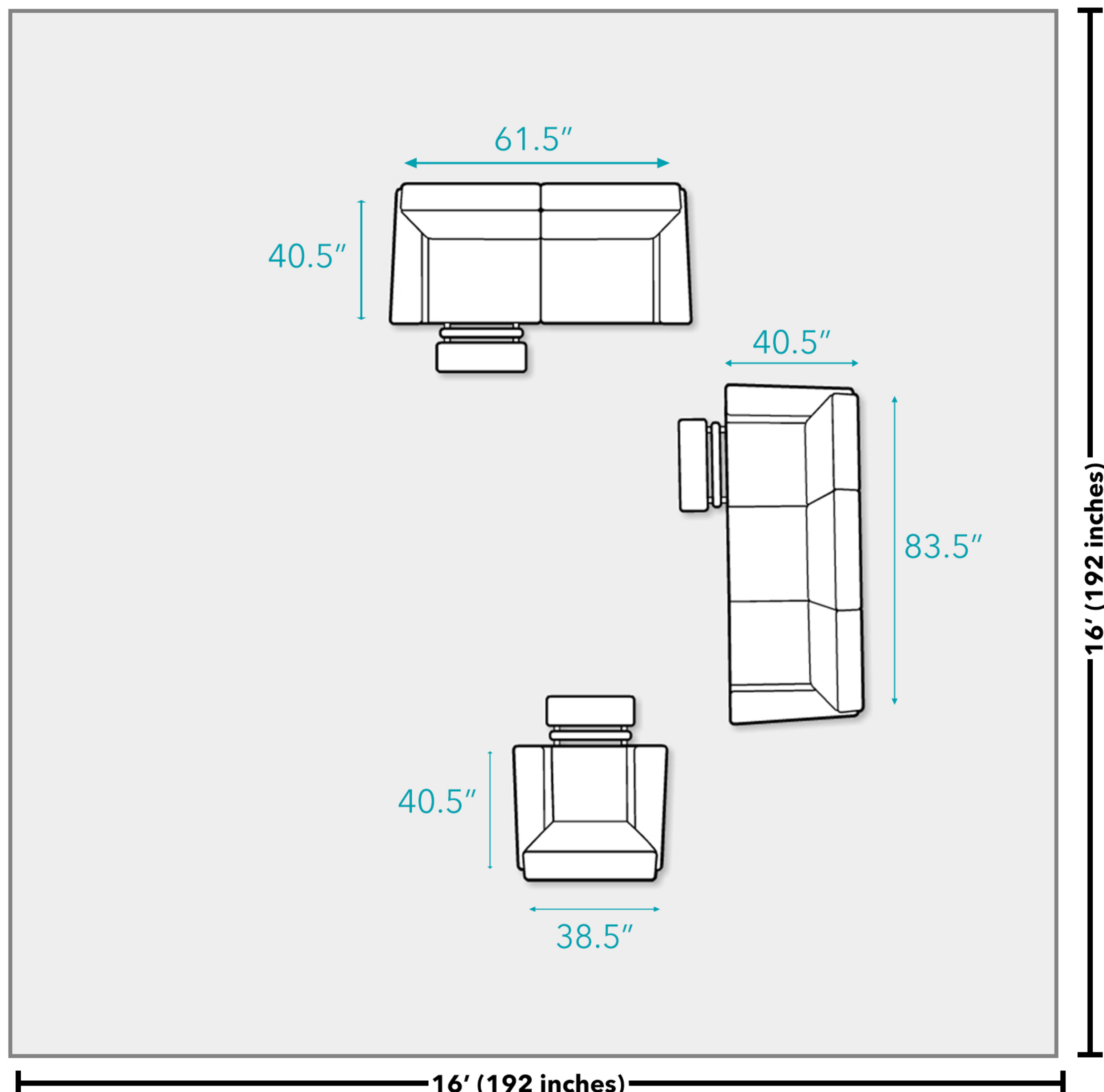
Floor Plan
