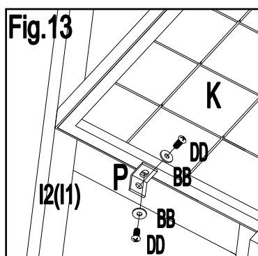
Fig 13: Put Table Top (K) on the assembled Screen, and fix it on Post 1&2 (I1&I2) by Corner Slice (P), Bolt (DD) and Washer (BB).
